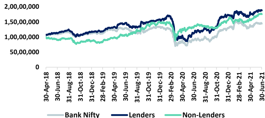
Backtest of Lenders & Non-Lenders in KCP (Apr '18 - Jun '21)
